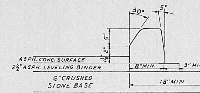
STANDARD DETAIL FOR 8" EXTRUDED CONC. CURB Not To Scale
