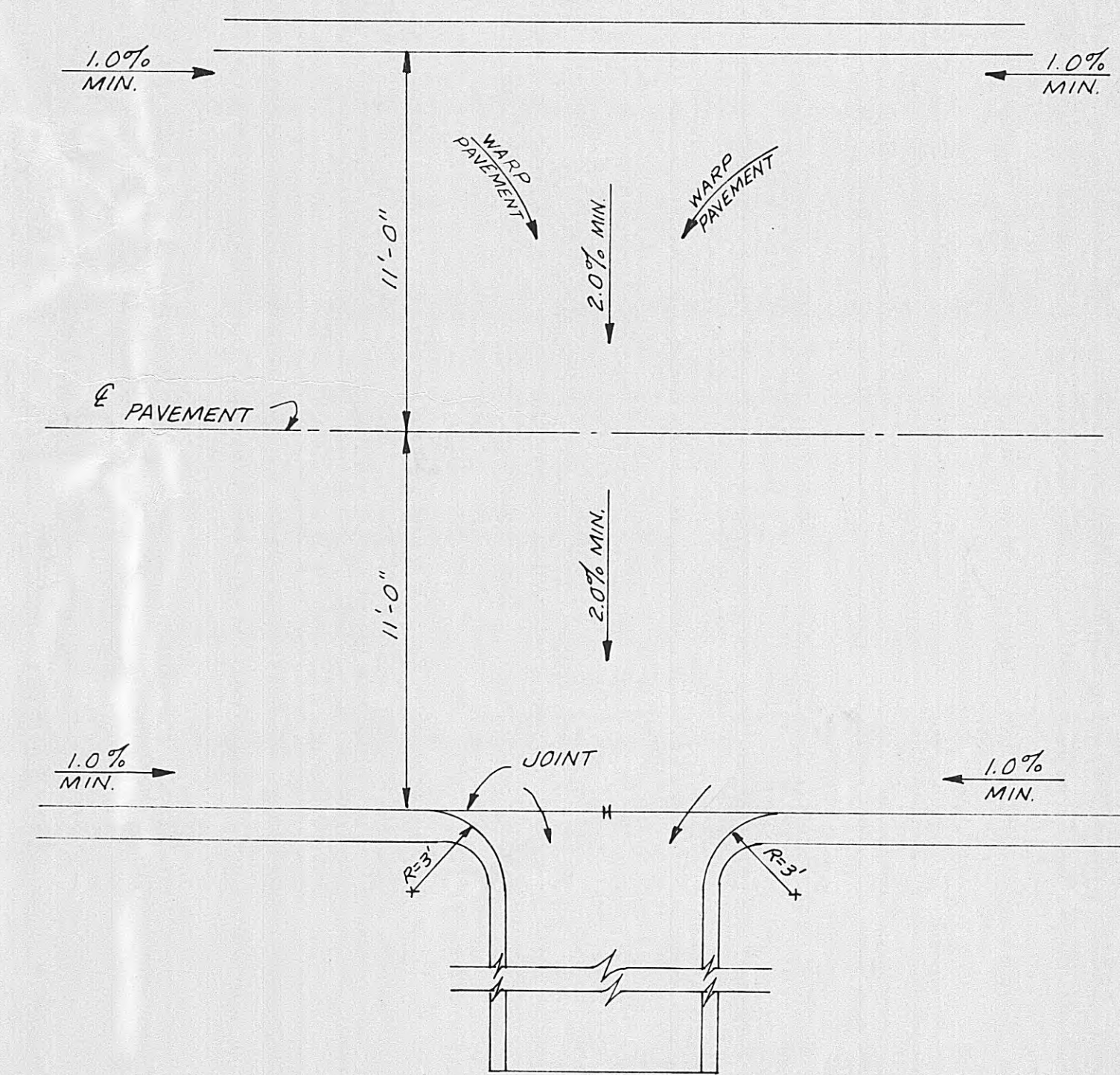
PAVING DETAIL - SINGLE SPILLWAY SCALE: 1" = 5'
