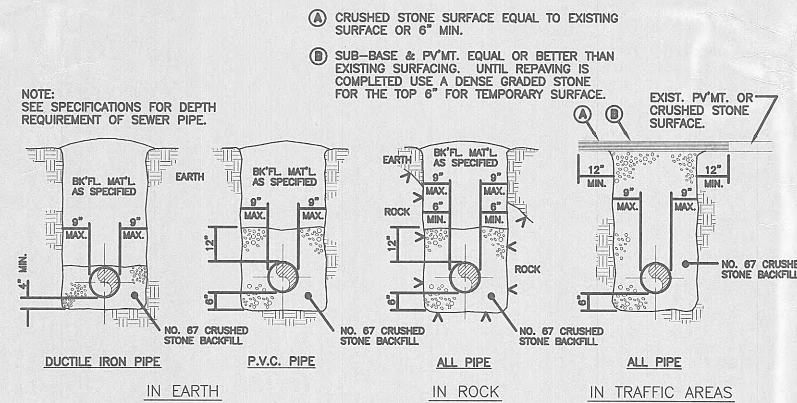
STANDARD GRAVITY SEWER BEDDING AND BACKFILLING NOT TO SCALE
