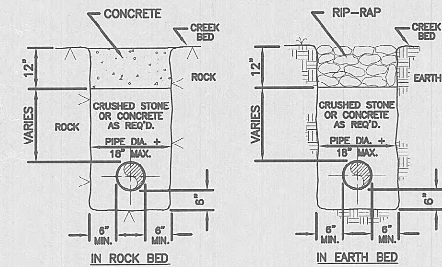
STANDARD CREEK CROSSING DETAIL NOT TO SCALE
