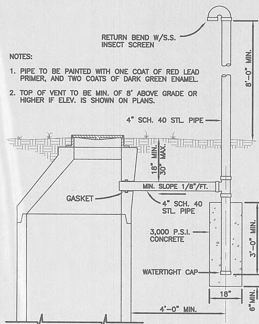
STANDARD MANHOLE VENT NOT TO SCALE
