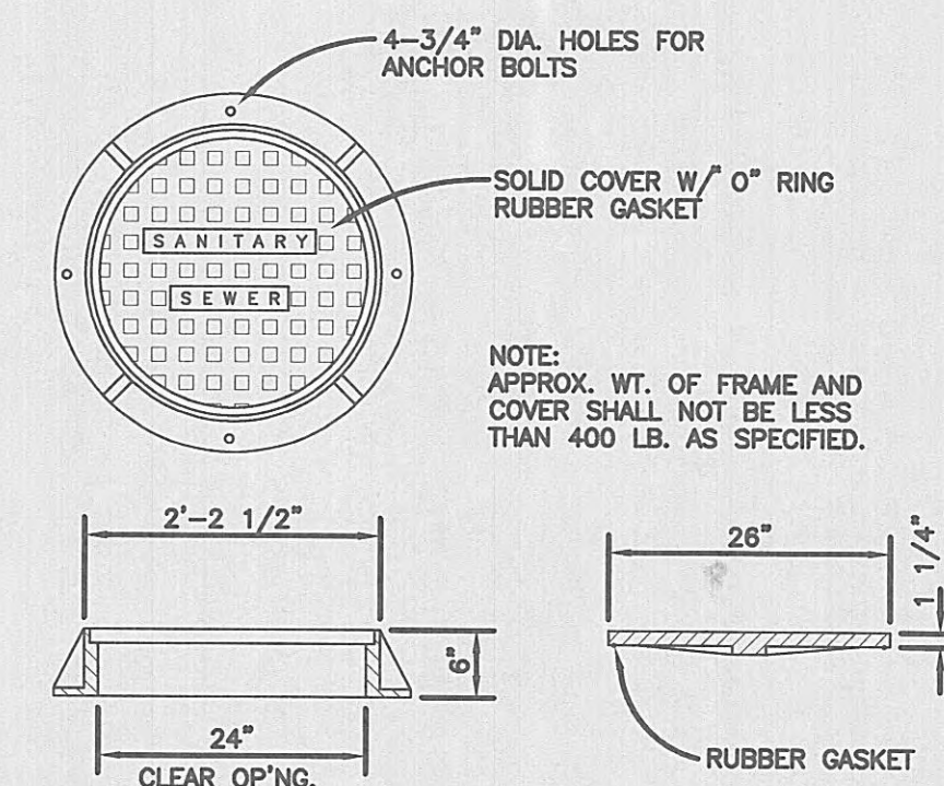
STANDARD MANHOLE FRAME & COVER NOT TO SCALE
