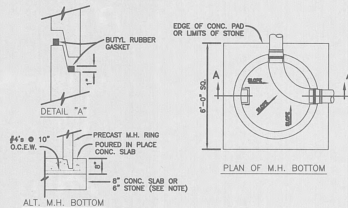
STANDARD MANHOLE NOT TO SCALE
