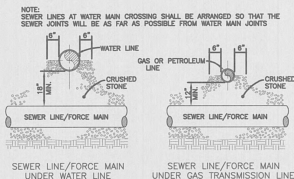
PIPE CROSSING FOR SEWER LINE/FORCE MAIN NOT TO SCALE
