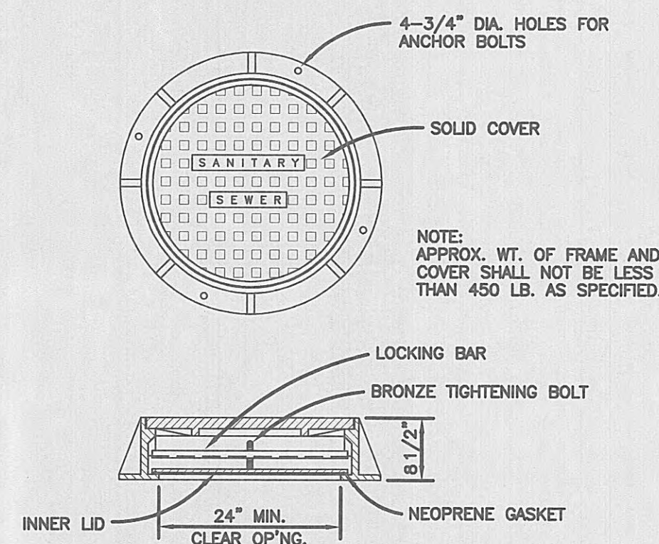
WATERTIGHT FRAME & COVER NOT TO SCALE
