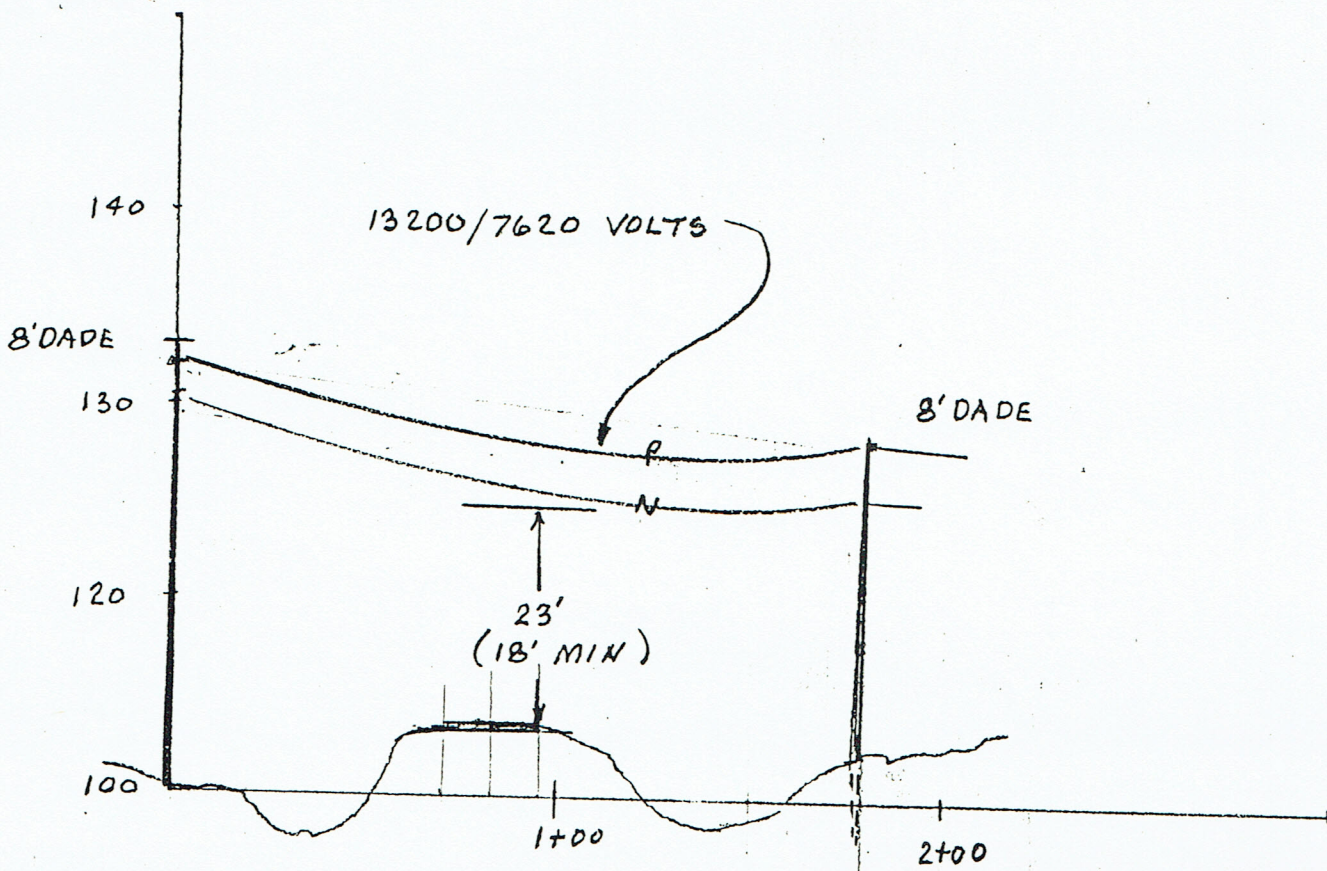
PROFILE
