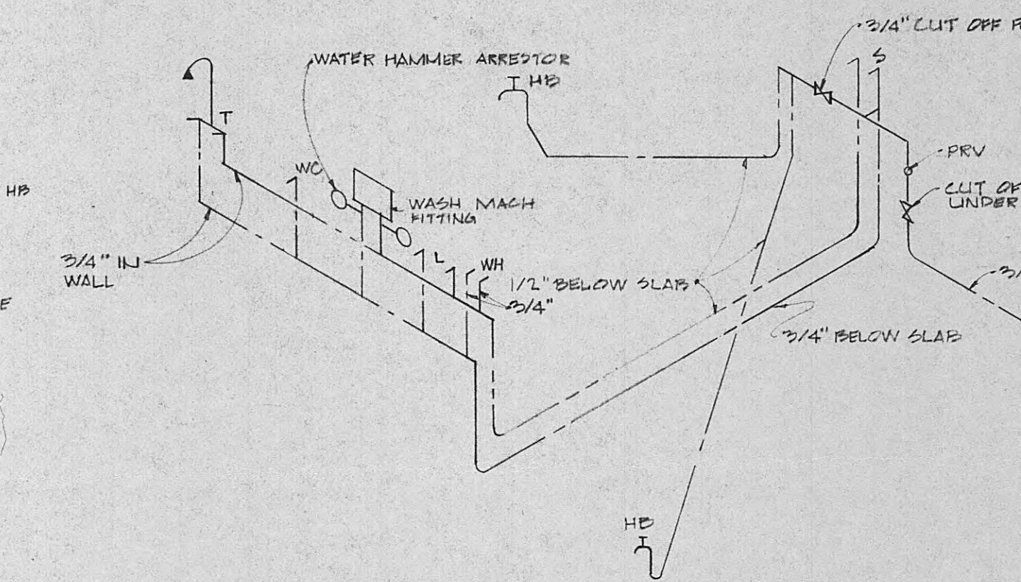
WATER PIPING TYPE E UNIT RIGHT END FOR UNIT OPPOSITE HAND
