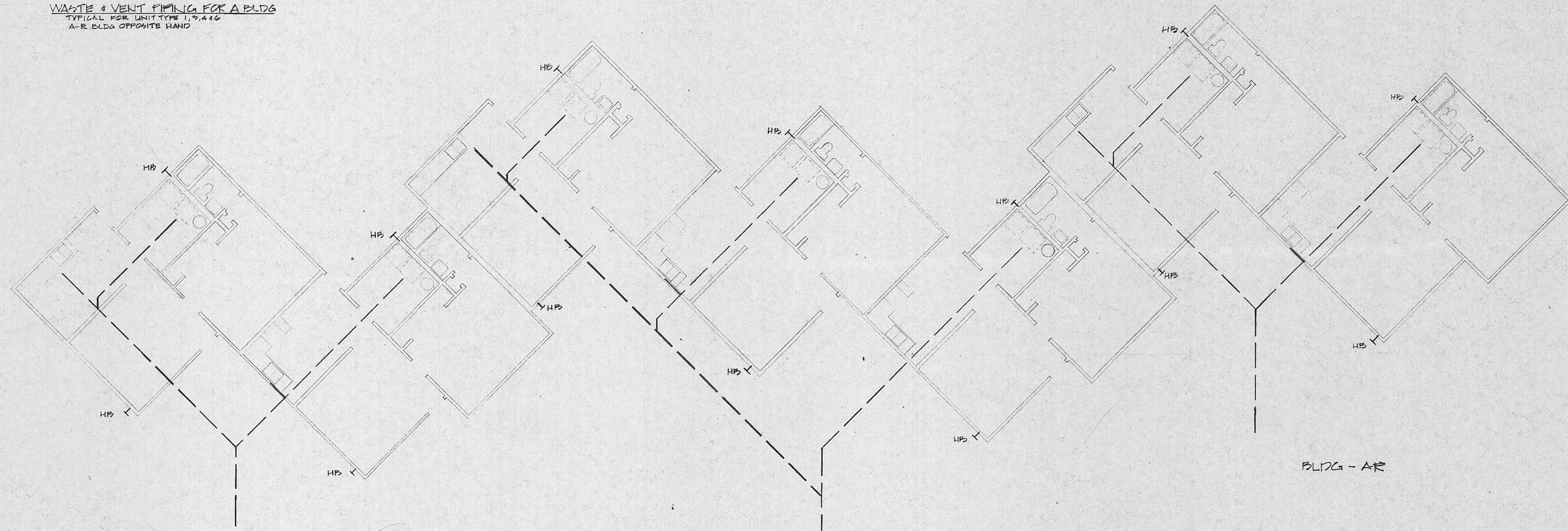
WASTE & VENT PIPING FOR A BLDG TYPICAL FOR UNIT TYPE 2, 3, 4 & 6 A-R BLDG OPPOSITE HAND
