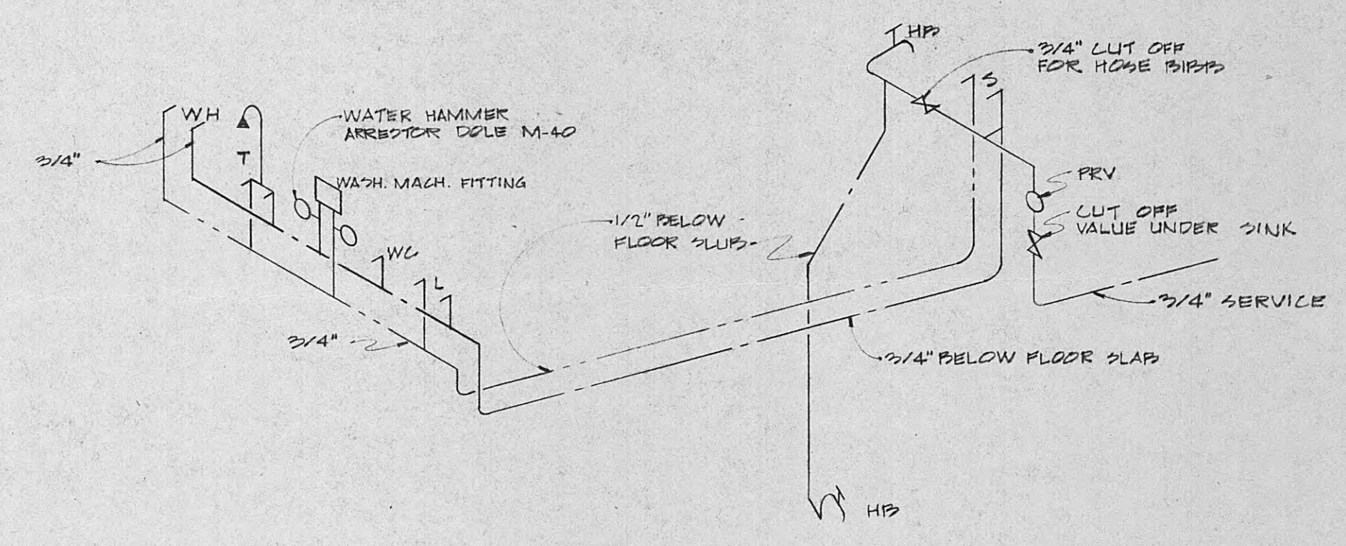
WATER PIPING TYPE C UNIT RIGHT END C-R UNIT OPPOSITE HAND
