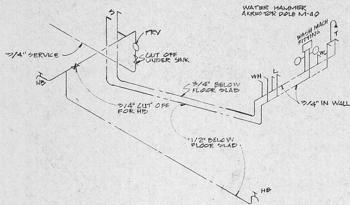
WATER PIPING TYPE D UNIT LEFT END FOR UNIT OPPOSITE HAND
