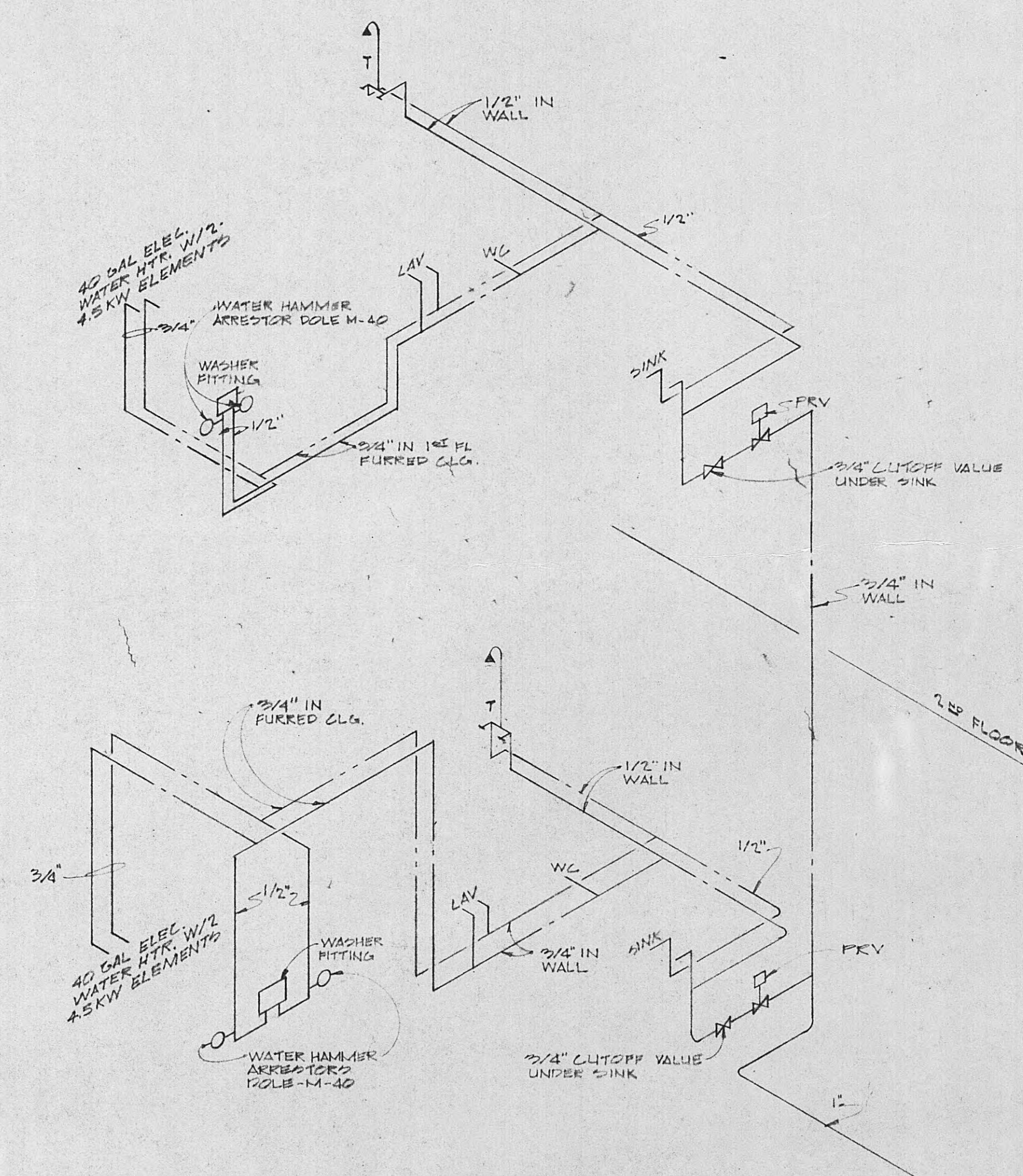
WATER ISOMETRIC - END UNITS "Q" ELDERLY BLDG
