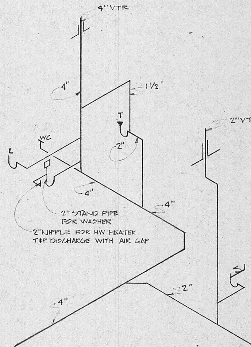
WASTE & VENT PIPING D UNIT RIGHT END FOR UNIT OPPOSITE HAND
