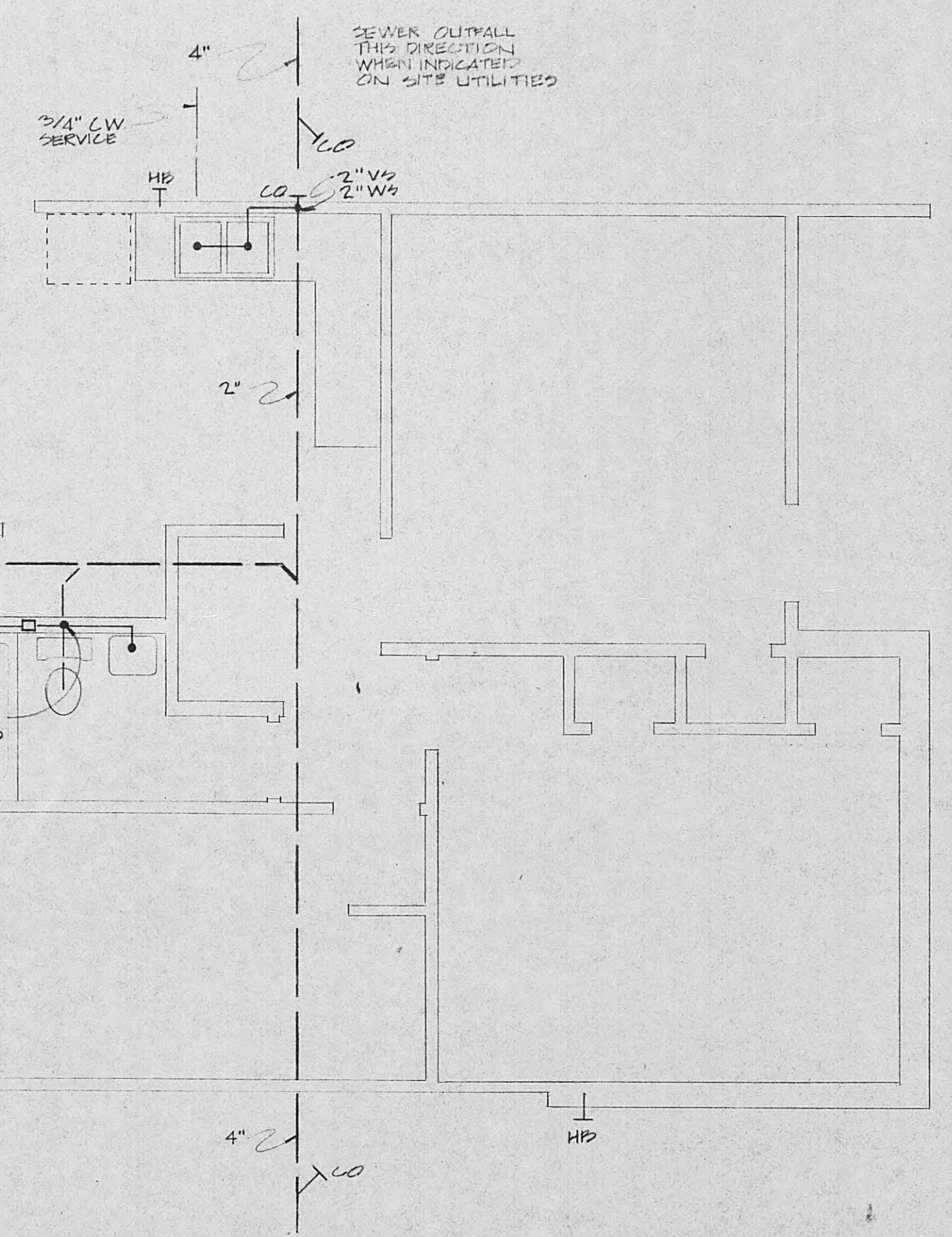
FLOOR PLAN TYPE C 1/8" = 1'-0"
