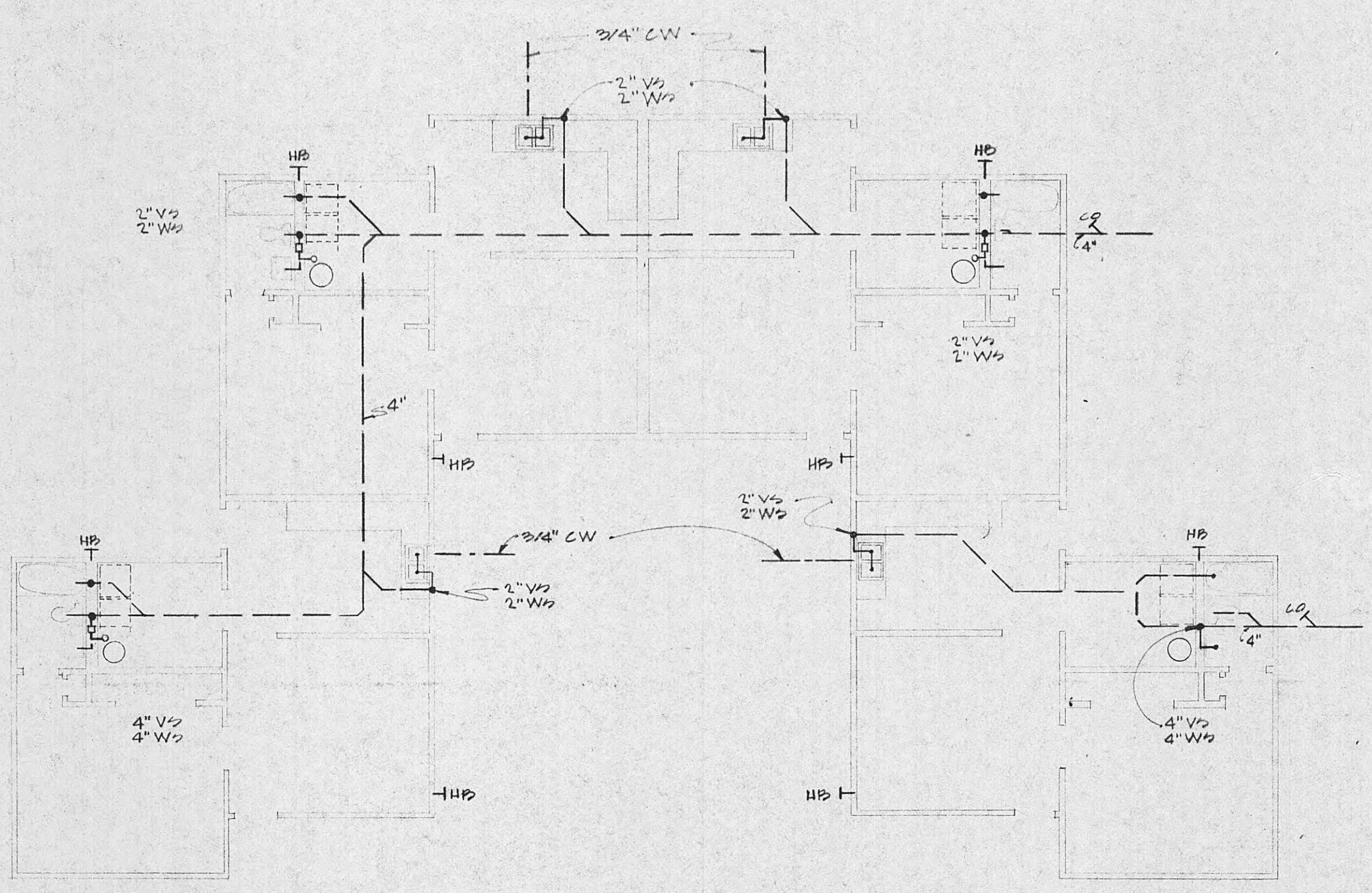
FLOOR PLAN TYPE B 1/8" = 1'-0"
