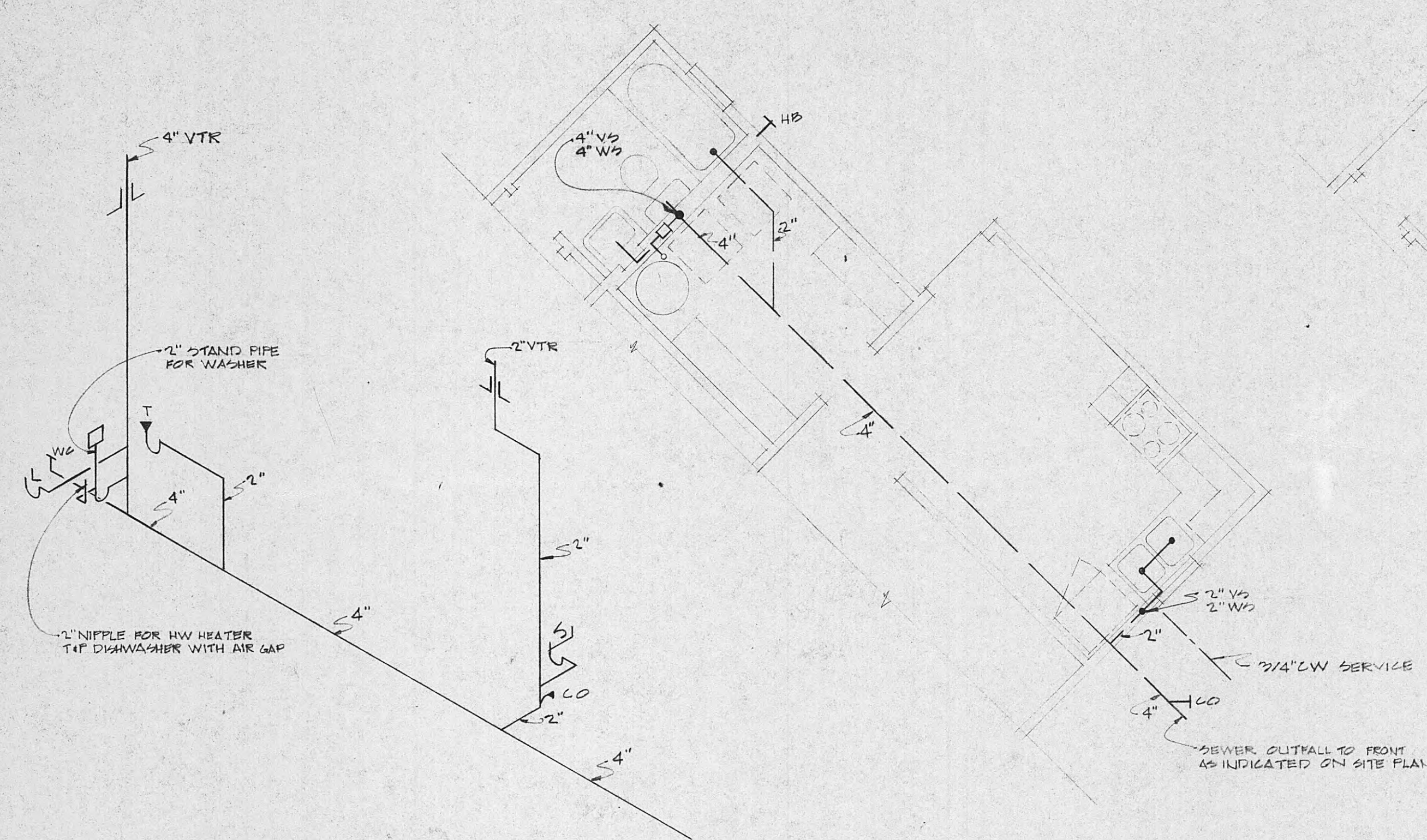
WASTE & VENT PIPING FOR A BLDG TYPICAL FOR UNIT TYPE 1, 3, 4 & 6 A-R BLDG OPPOSITE HAND
