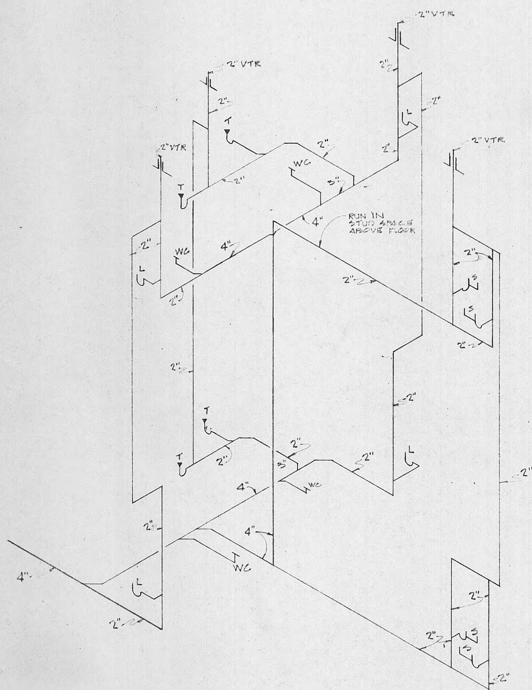
WASTE & VENT PIPING "Q" & "I" UNITS
