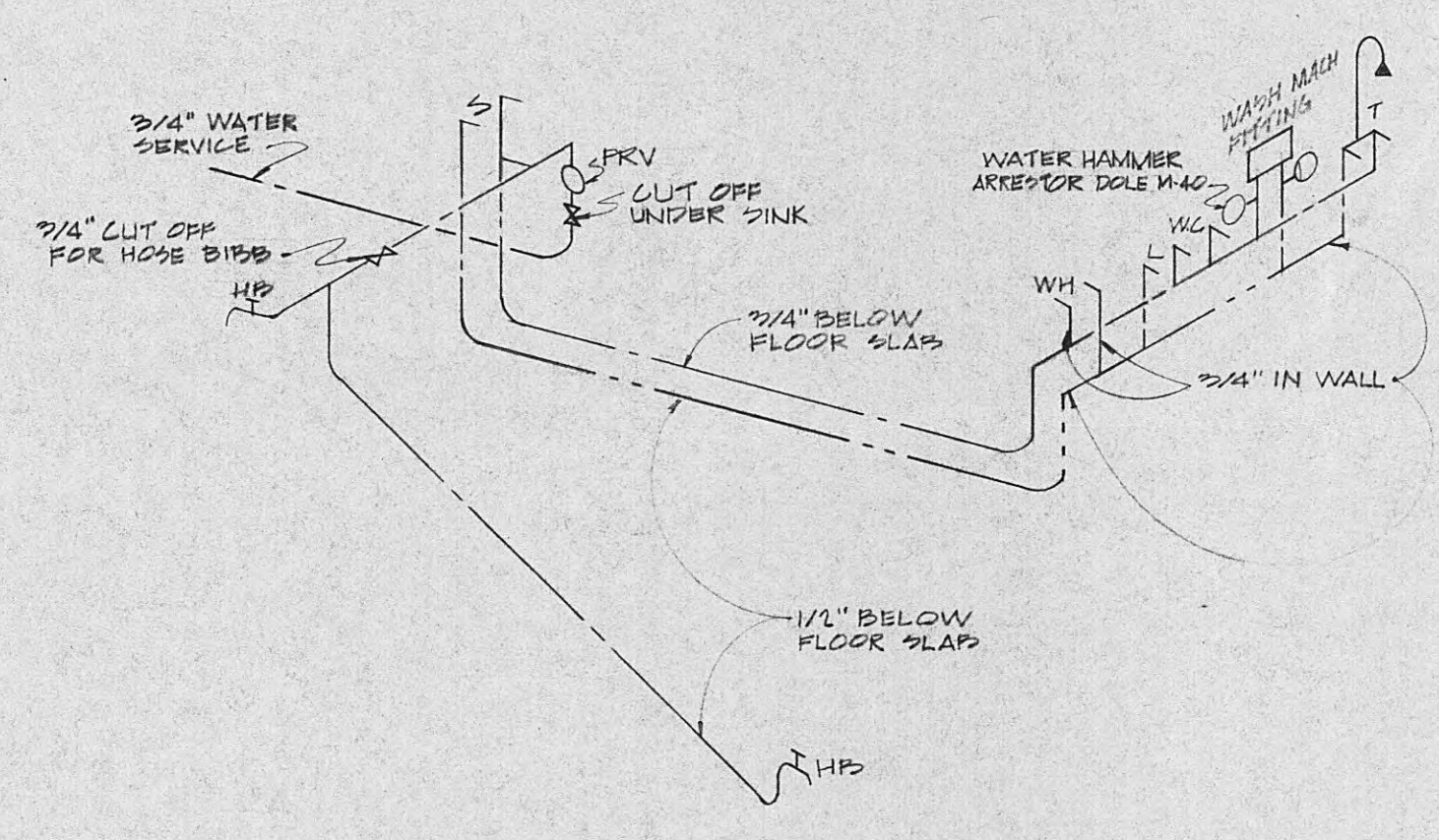
WATER PIPING TYPE C UNIT LEFT END C-R UNIT OPPOSITE HAND
