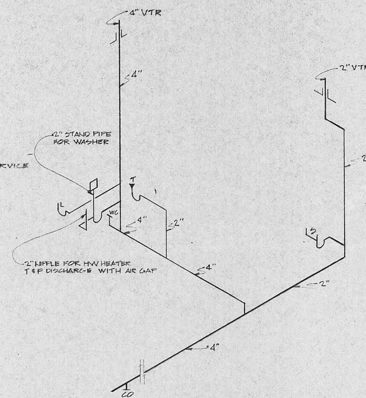
WASTE & VENT PIPING FOR A BLDG TYPICAL FOR UNIT TYPE 2, 3, 4 & 6 A-R BLDG OPPOSITE HAND
