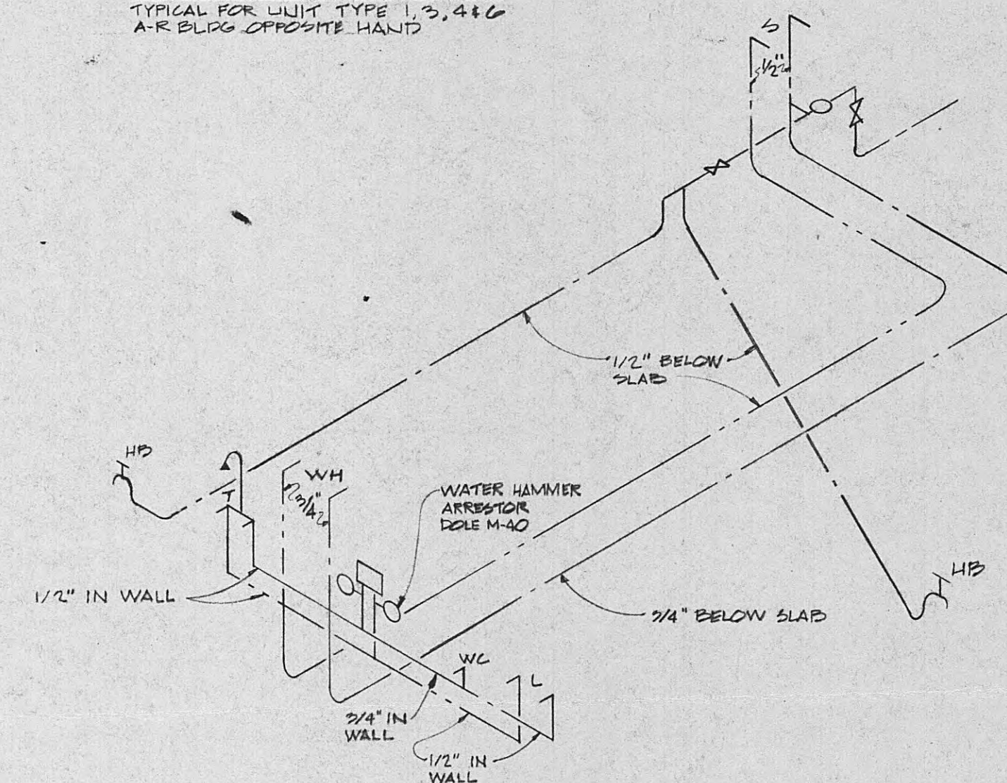
WATER PIPING FOR A BLDG TYPICAL FOR UNIT TYPE 1, 3, 4 & 6 A-R BLDG OPPOSITE HAND
