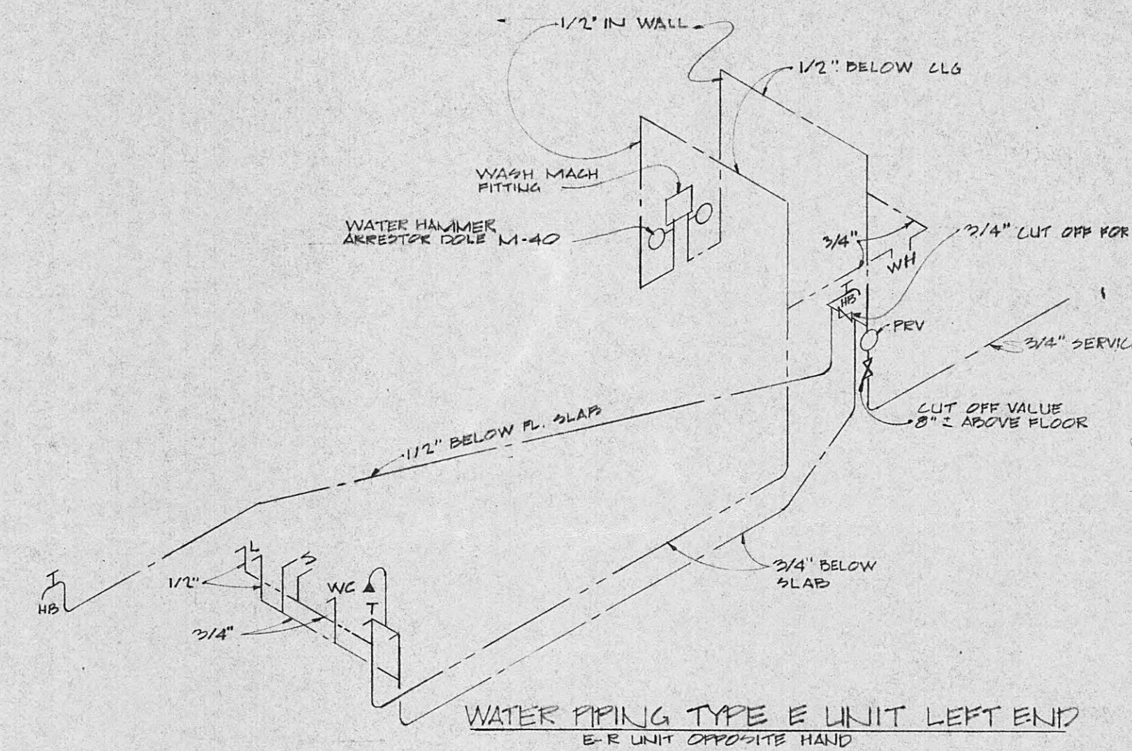
WATER PIPING TYPE E UNIT LEFT END FOR UNIT OPPOSITE HAND
