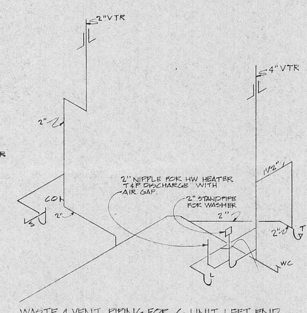
WASTE & VENT PIPING FOR C UNIT LEFT END C-R UNIT OPPOSITE HAND
