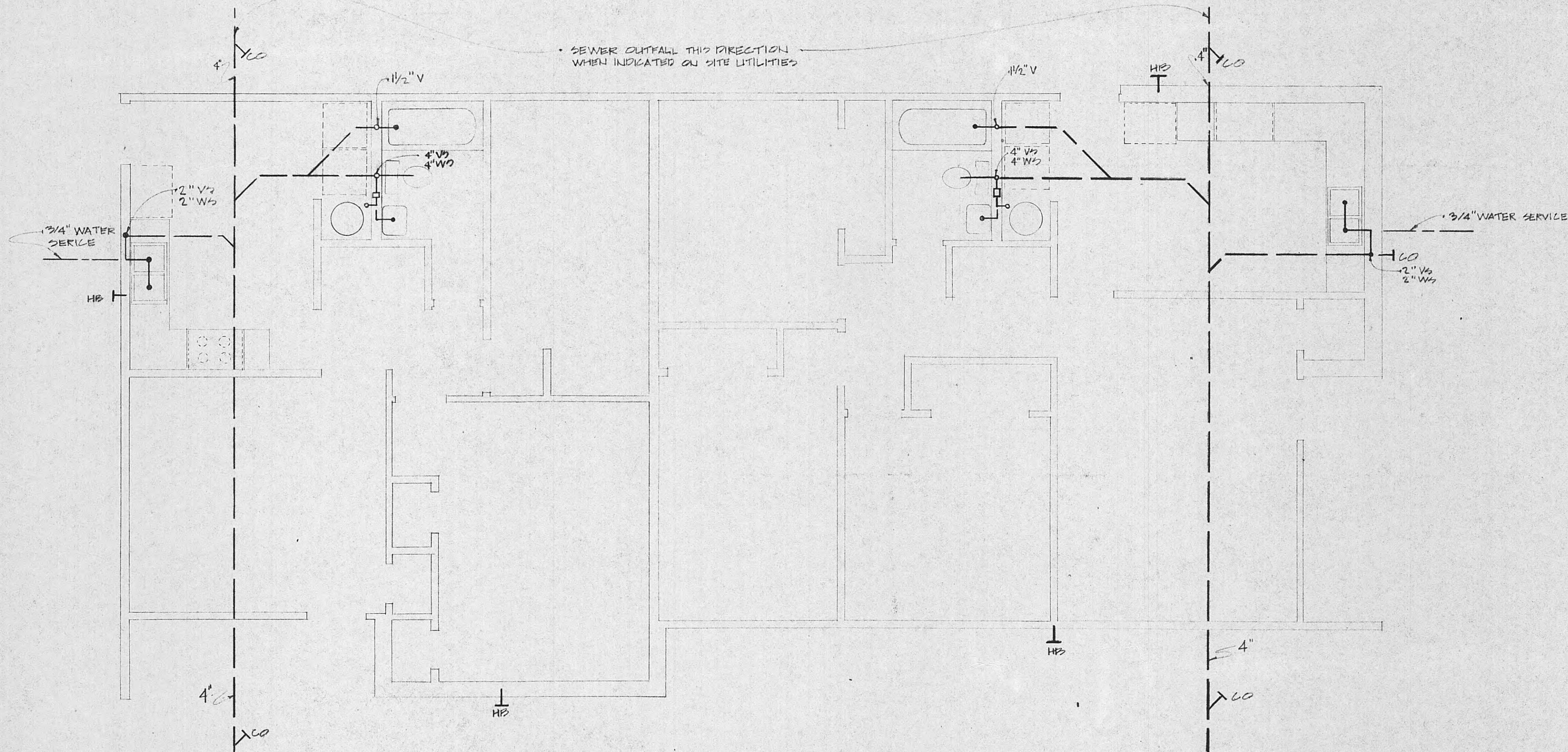
FLOOR PLAN TYPE "D" 1/4" = 1'-0"
