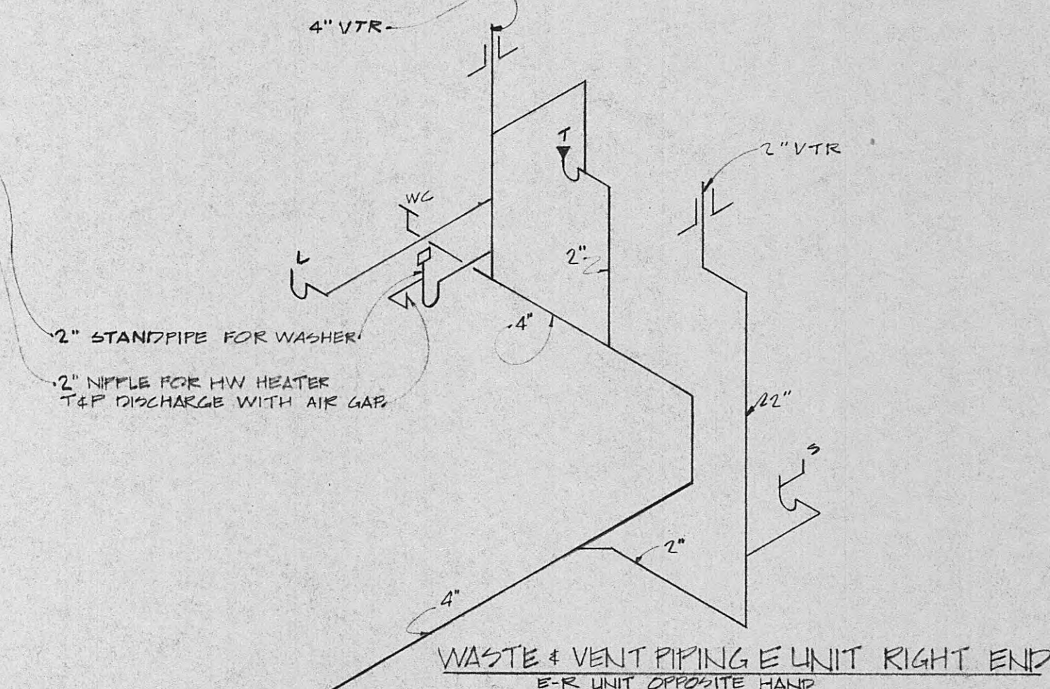
WASTE & VENT PIPING E UNIT RIGHT END FOR UNIT OPPOSITE HAND
