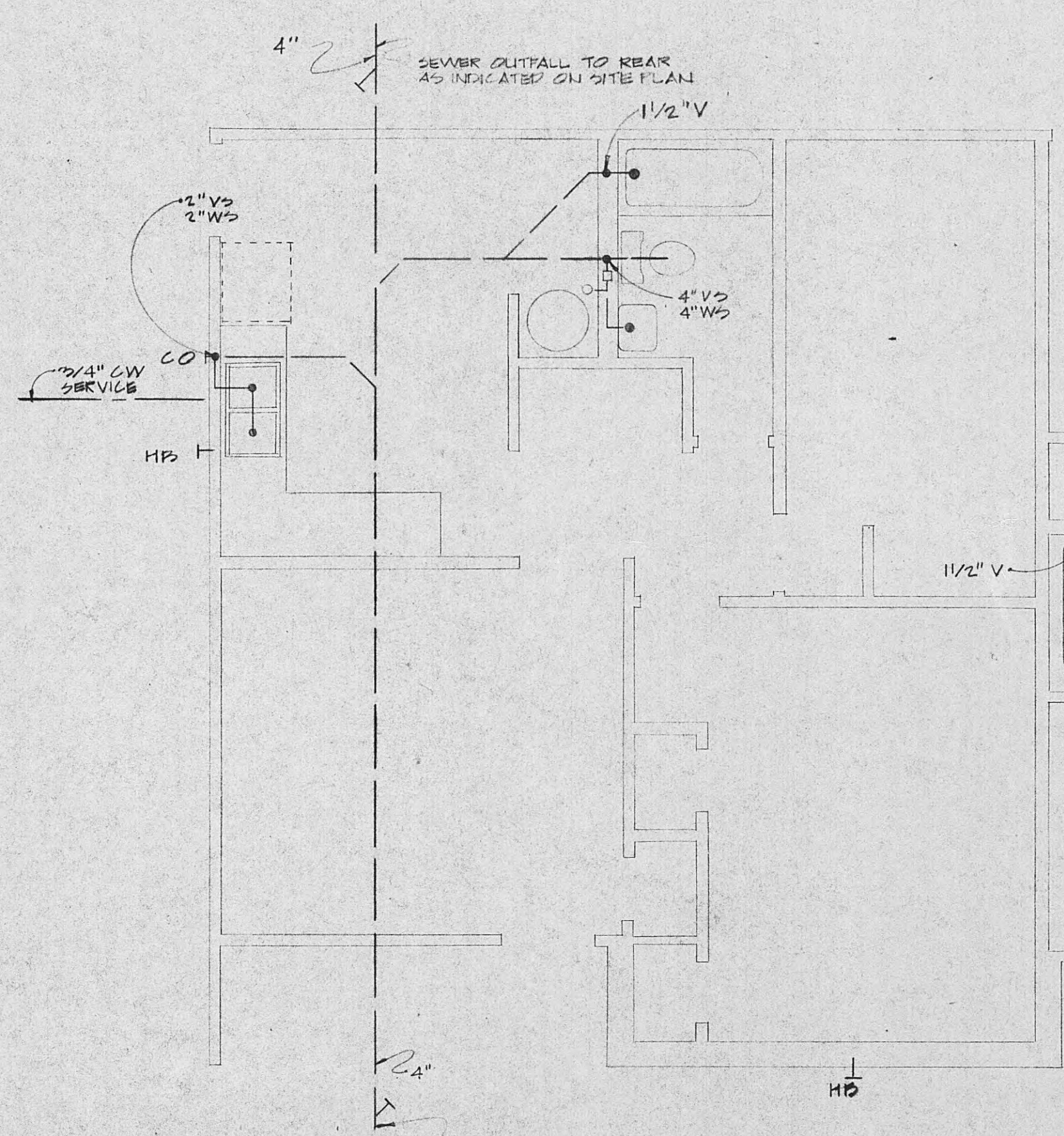
SEWER OUTFALL TO FRONT AS INDICATED ON SITE PLAN
