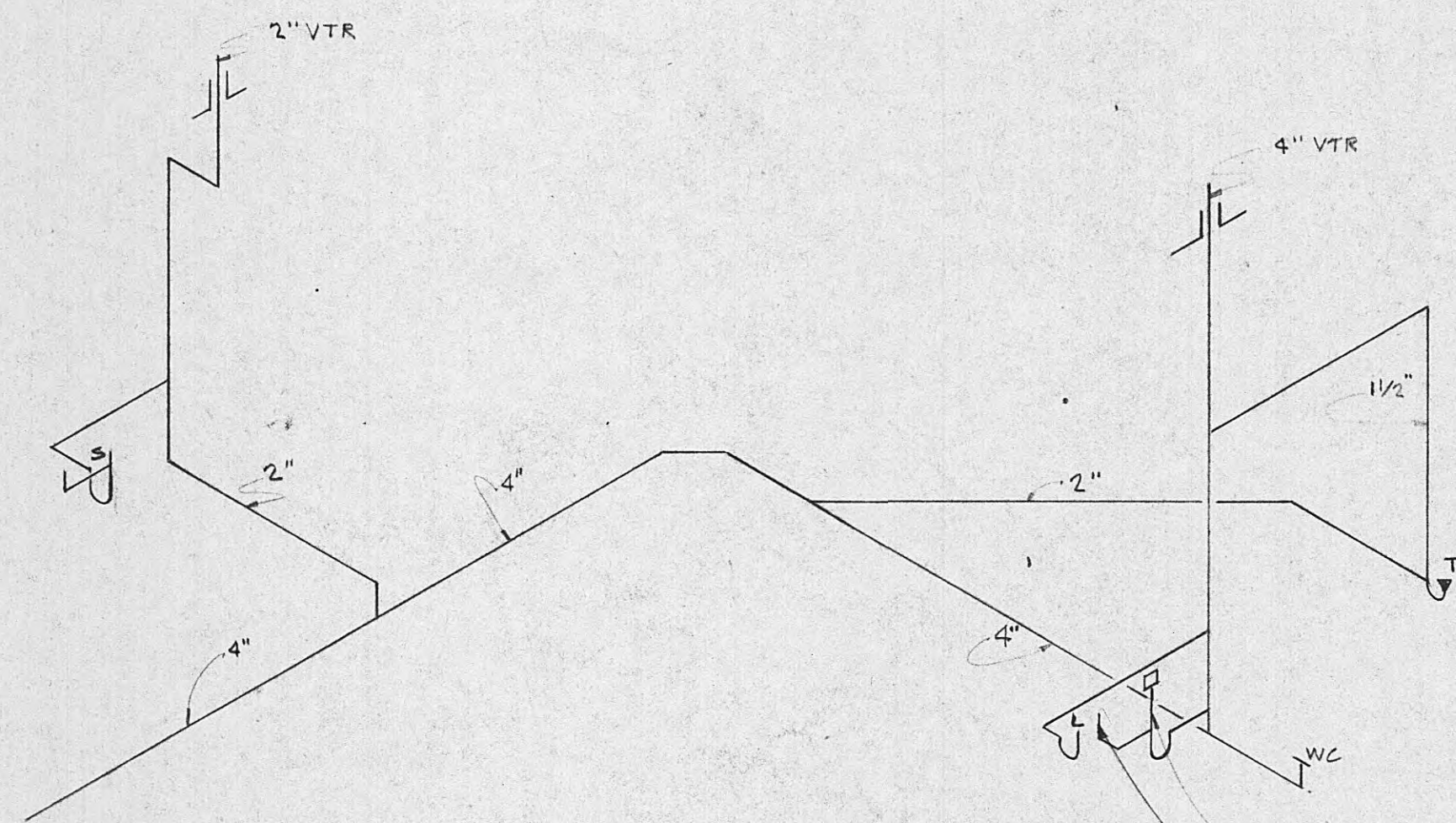
WASTE & VENT PIPING D UNIT LEFT END FOR UNIT OPPOSITE HAND
