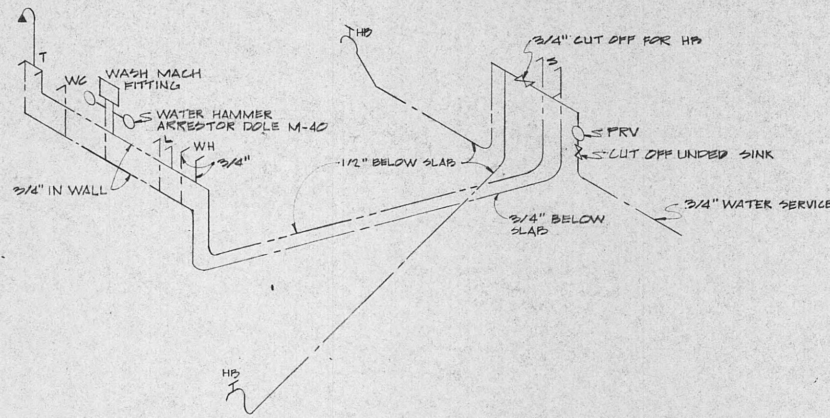
WATER PIPING TYPE D UNIT RIGHT END FOR UNIT OPPOSITE HAND
