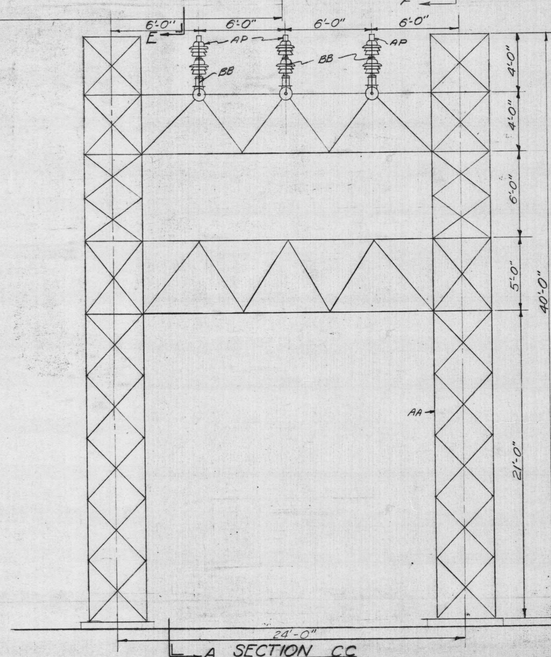
SECTION CC
