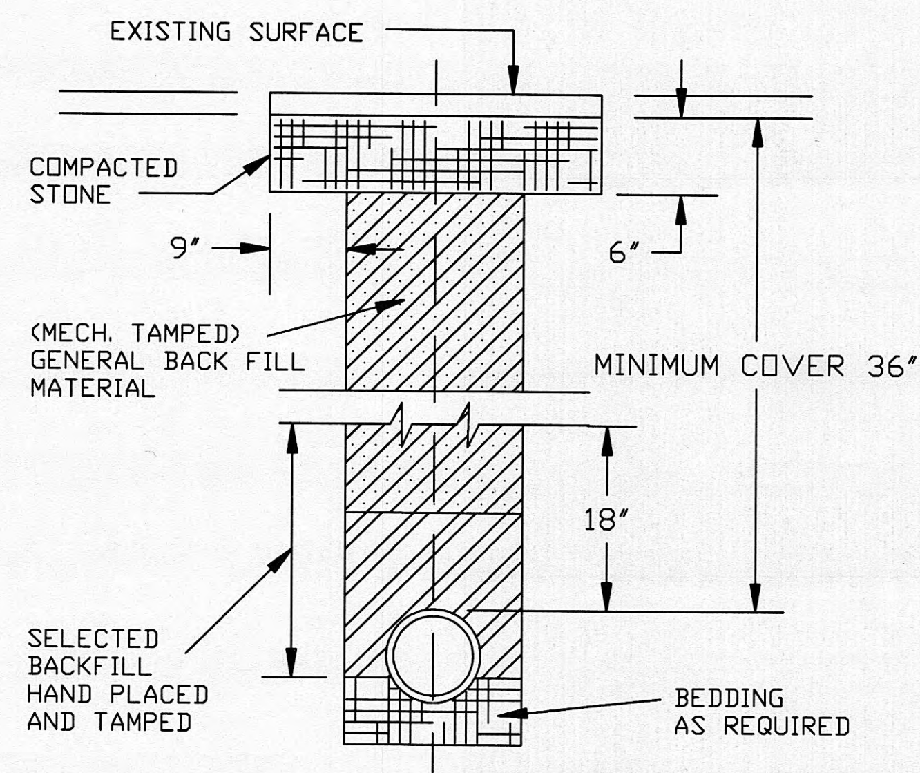
TYPICAL DITCH DETAIL
