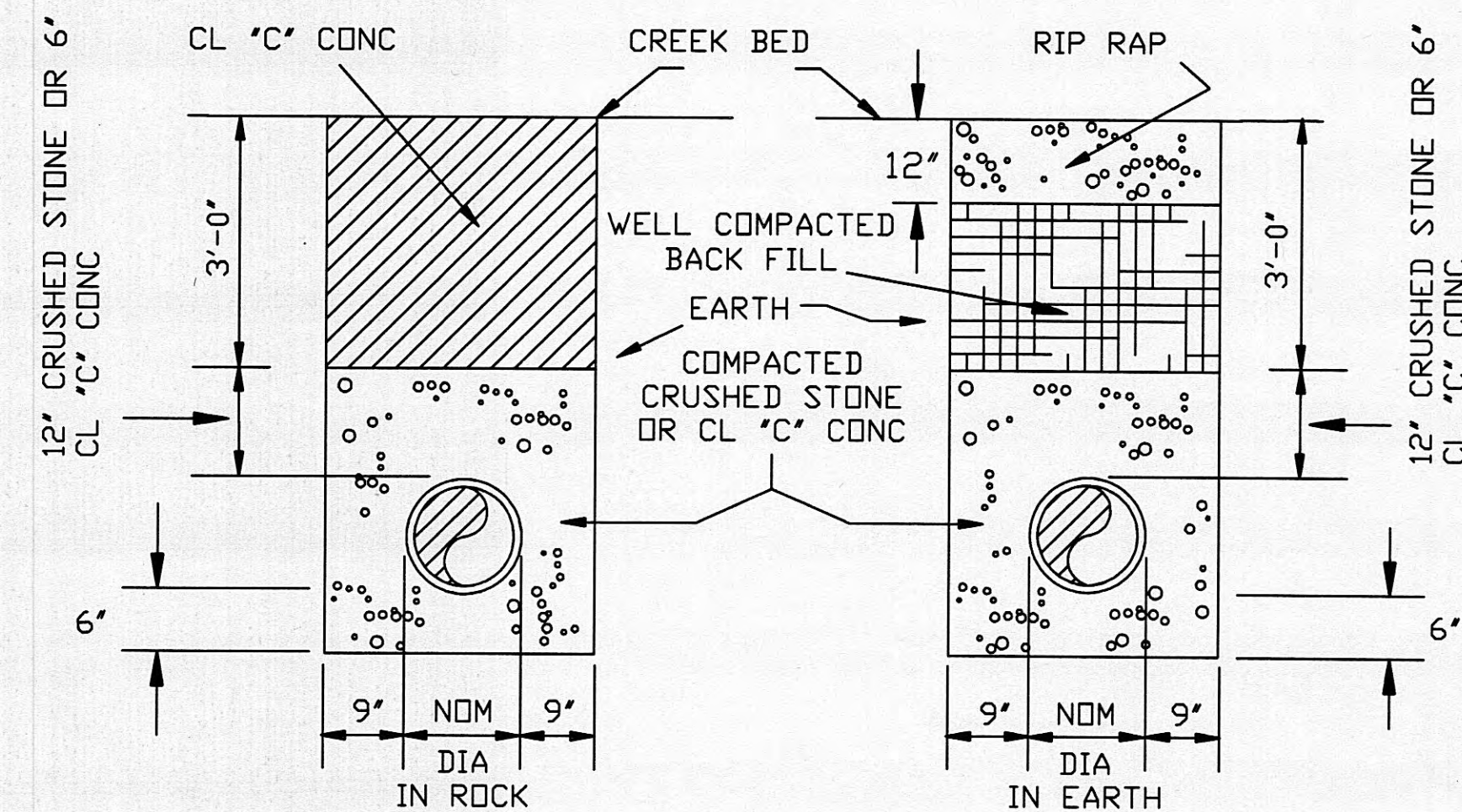
TYPICAL STREAM CROSSING DETAIL
