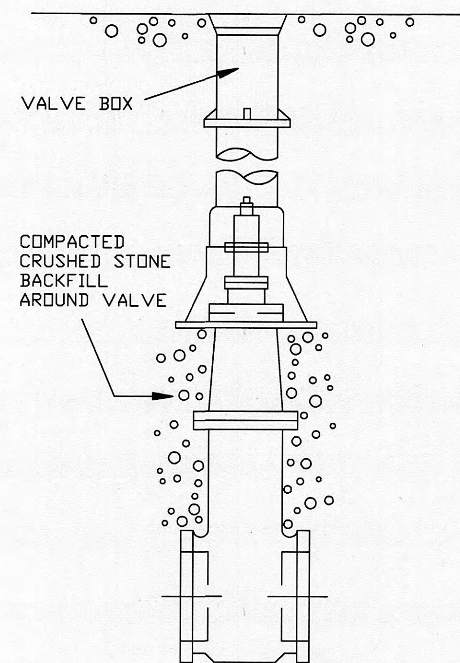
TYPICAL VALVE BOX DETAIL
