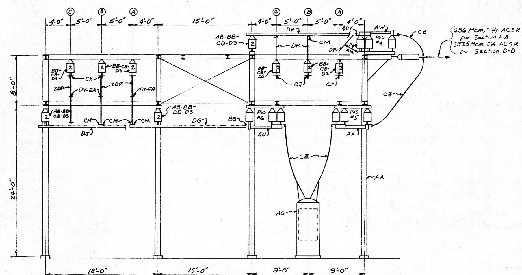
SECTION A-A 69 kv to Oliver Spring SECTION D-D 69 kv to Melton Hill Tap
