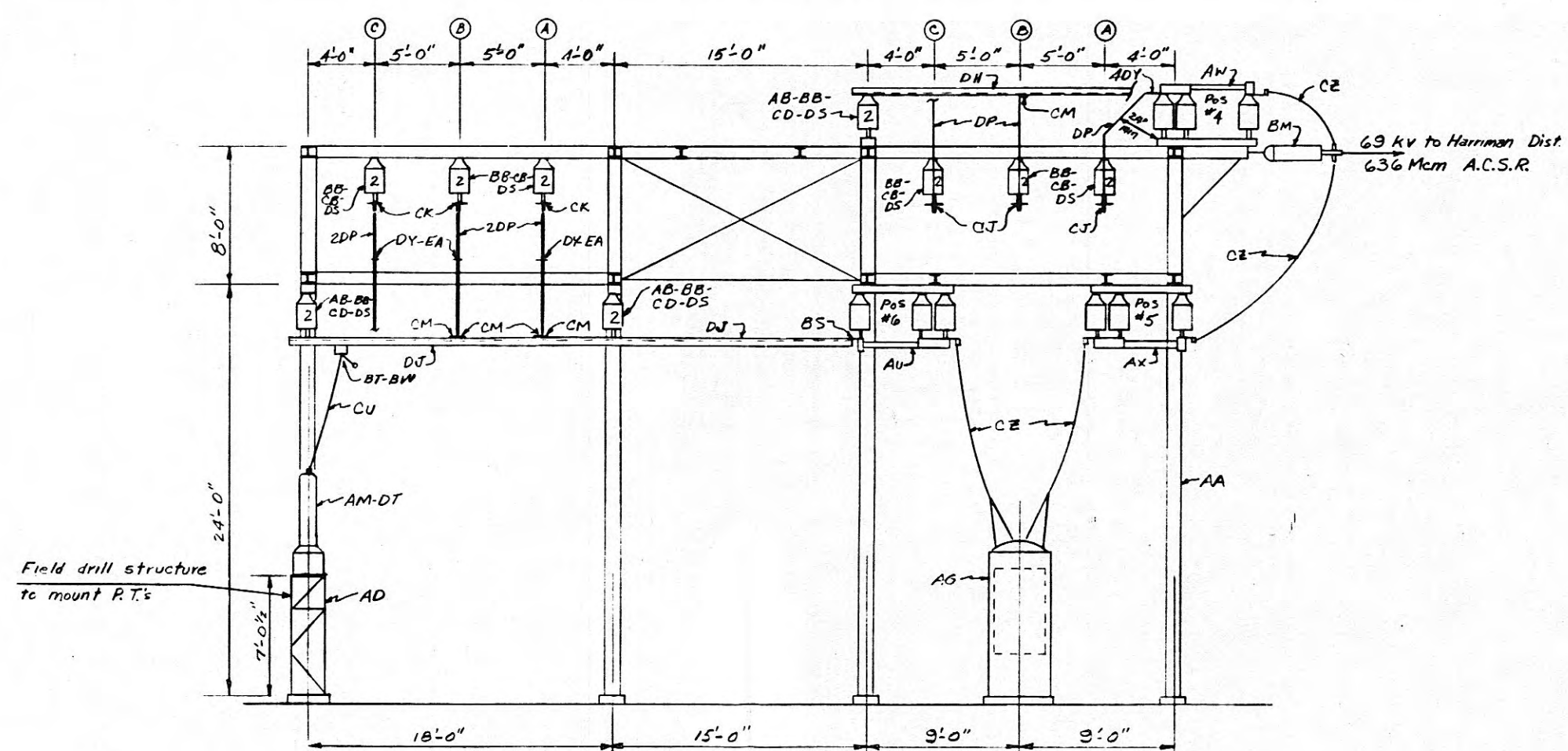
SECTION B-B
